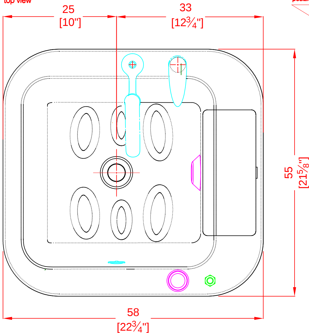
vista in pianta top view
